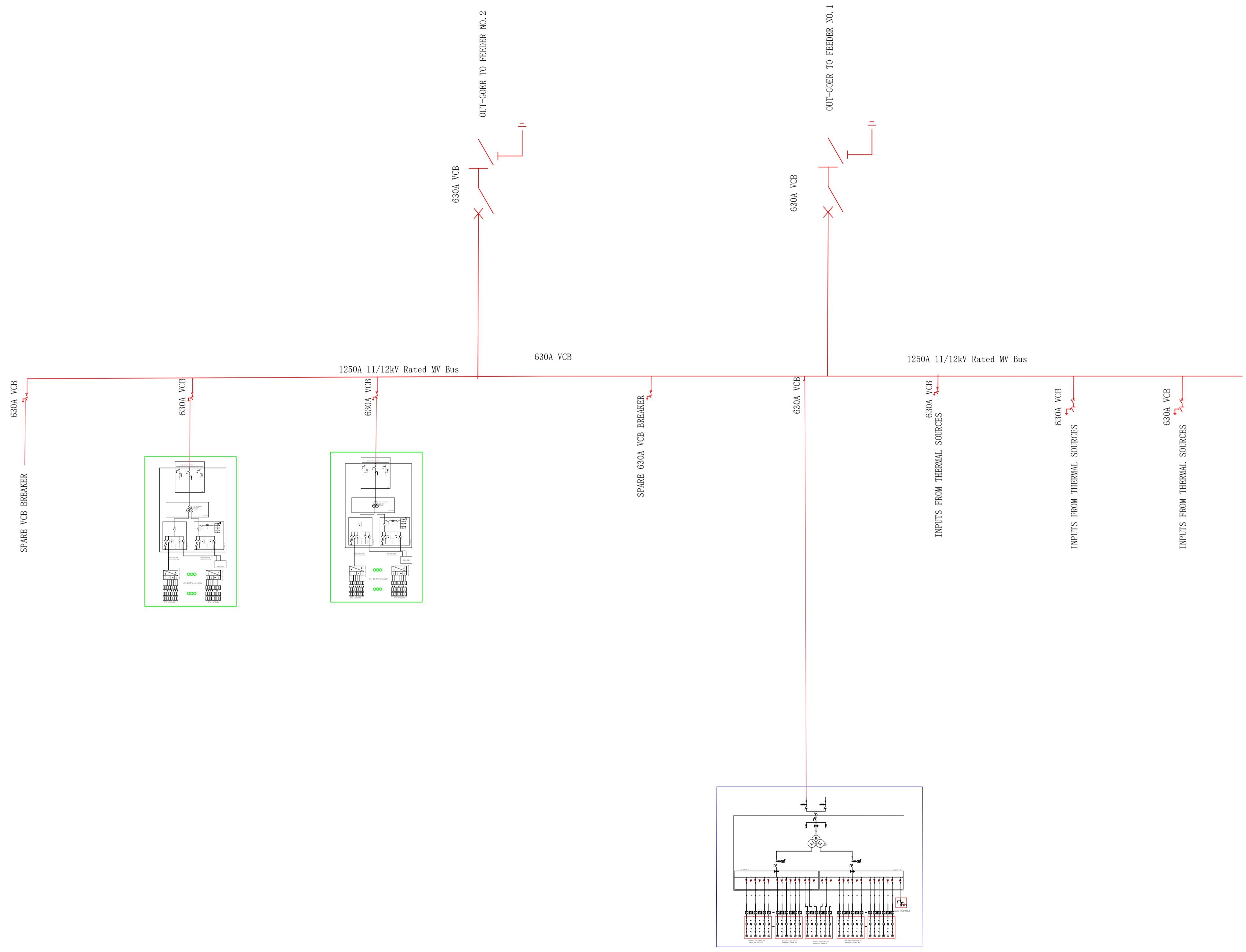
SINGLE LINE DIAGRAM FOR THE PROPOSED PV POWER PLANT FOR GECO ELECTRICITY SERVICE PROVIDE IN GALKA'YO, SOMALIA
