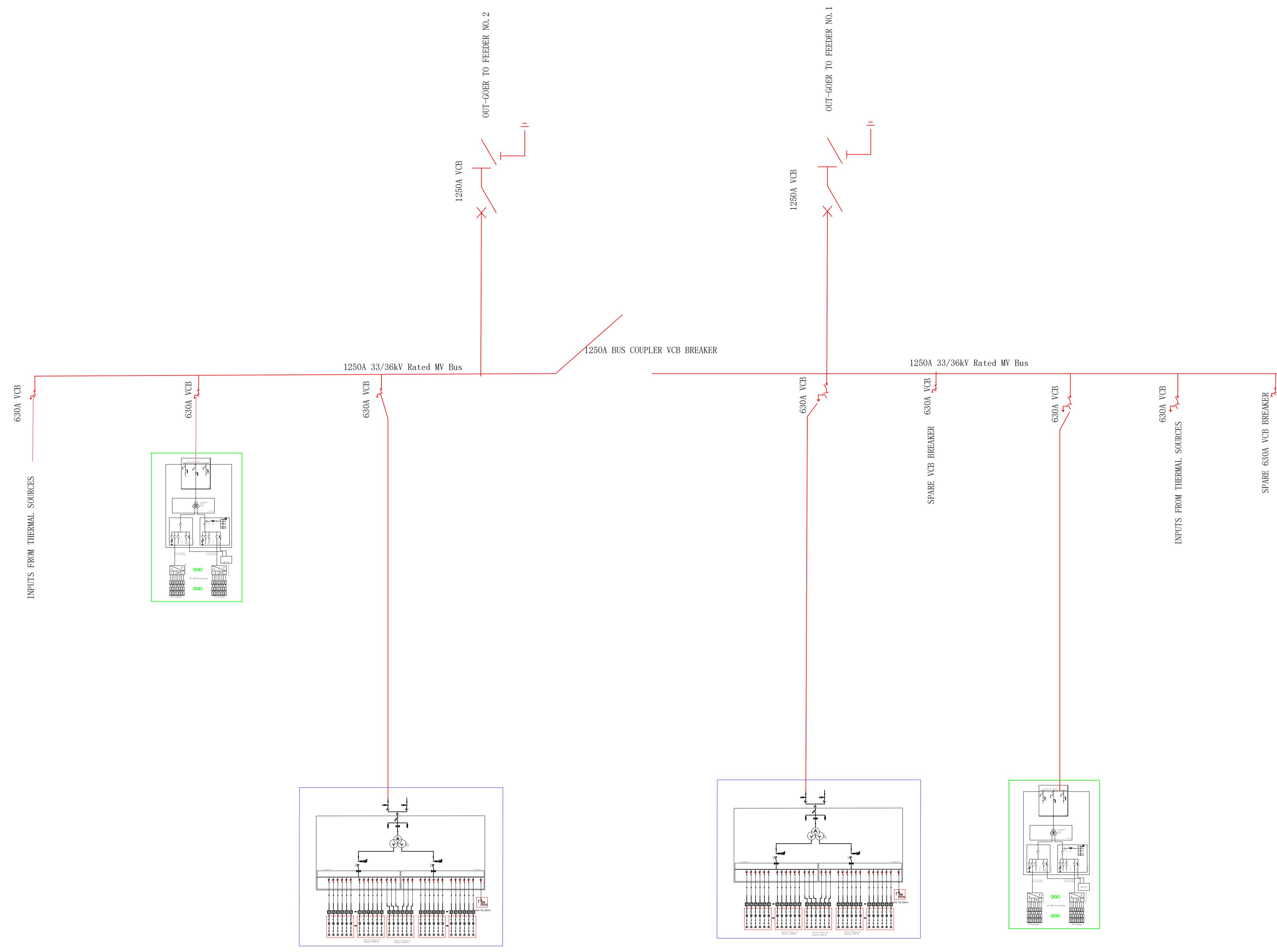
SINGLE LINE DIAGRAM FOR THE PROPOSED PV POWER PLANT FOR NEPCO ELECTRICITY SERVICE PROVIDE IN GALKA'YO, SOMALIA
